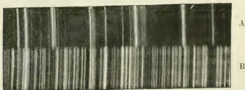
FIG. 8.—Parts of the spectra of (A) barium and (B) iron (from a photograph).
